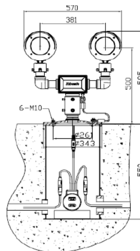
Installation method II: Coordinated with base L-867
