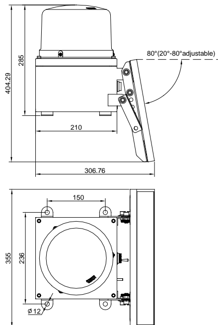
Angle 80° installation diagram
