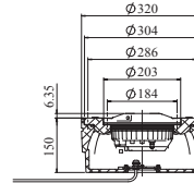
Fig 2. On 12" shallow base w/ 12"/8" adapter ring
