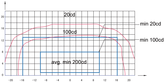
SBLMS-08-LED (Red), ICAO Figure A2-12
