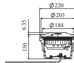
Fig 1. On 8" shallow base
