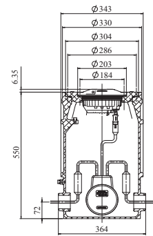
Fig 3. On 12" deep base w/ 12"/8" adapter ring
